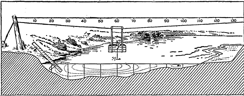
FIGURE 49.—Method of measuring the flow of a river at a cable station. The view shows the section of the river and the car, gage, and other apparatus.
