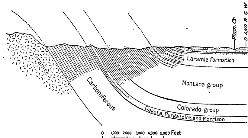
FIGURE 6.—Section at mouth of Platte Canyon.
