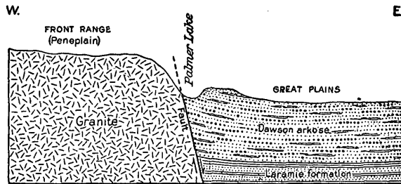
FIGURE 8.—Sketch section through Palmer Lake, showing fault. The granite on the west has moved up (see Pl. LXXXVII, p. 216) with reference to the rocks of the plains.
