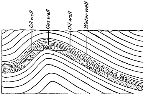
FIGURE 38.—Relation of oil, gas, and water to an anticline. In a porous sandstone gas may be forced to the top of the arch, oil will come next, and water will lie in the lower part.
