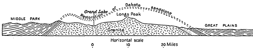
FIGURE 3.—Arch of the Front Range restored. After Lee.
