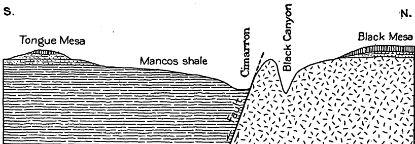
FIGURE 46.—Section across Black Canyon at Cimarron. The rocks have broken along the fault shown in the section, and the granite on the north has been forced up far above its original position.
