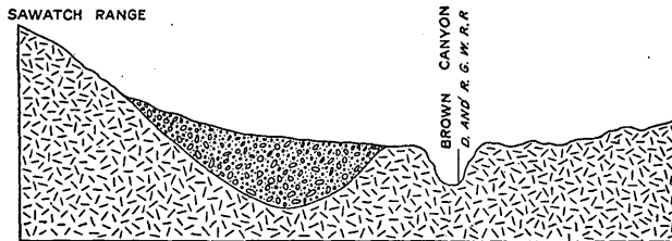
FIGURE 20.—Ideal section from Sawatch Range to Brown Canyon, showing the deep gravel filling in the old channel of the Arkansas.
