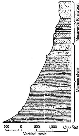
FIGURE 57.—Geologic section at Castlegate.
