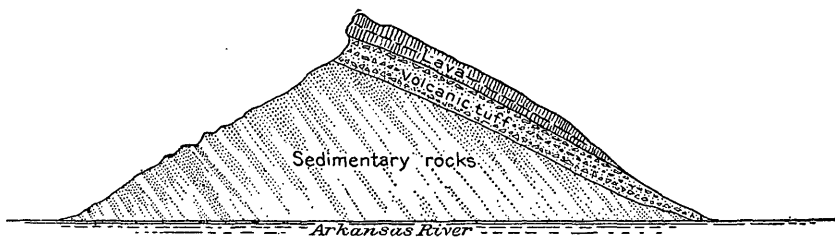
FIGURE 18.—Lava-capped hill south of Howard. The hill, which is opposite milepost 200, is composed of red sandstone dipping steeply to the northwest and is capped by a nearly horizontal sheet of tuff and lava.
