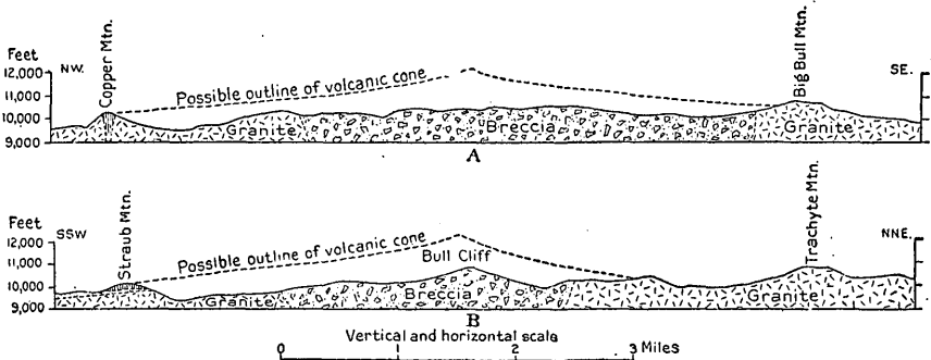
FIGURE 12.—Sections showing supposed outline of the Cripple Creek volcano.
