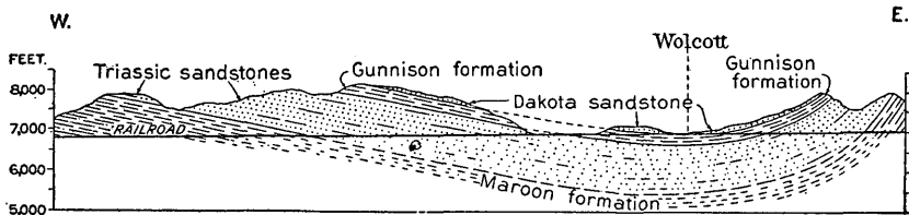
FIGURE 32.—Sketch section across the syncline at Wolcott on a line from east to west.
