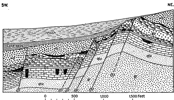
FIGURE 27.—Section through some of the workings at Leadville, showing the relation of the ore to the limestone, porphyry, and quartzite. wp, White porphyry; gp, gray porphyry; lvi., Leadville limestone; pq, parting quartzite; wl, white limestone; qtz, lower quartzite; gr, granite. The ore bodies are indicated by cross hatching. The straight heavy lines represent faults, and the arrows show the direction of movement.
