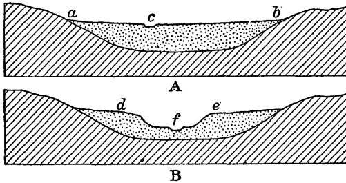
FIGURE 41.—Formation of a gravel terrace.
