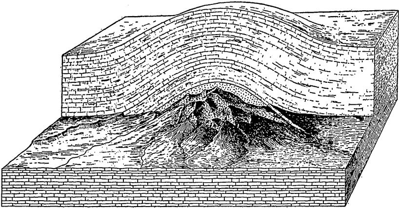
FIGURE 53.—Mountains carved from a laccolith. The block at the rear shows the former position of the sedimentary beds after they were forced upward by the intrusion of the lava.
