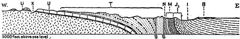
FIGURE 10.—Section through Garden of the Gods. The spires and walls of the gateway are carved in the upstanding block of sandstone, and this block is separated from the rocks on both sides by faults. For explanation of letters see Plate XXII.
