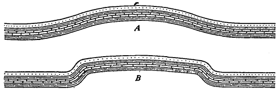
FIGURE 51.—Different types of anticlines.
