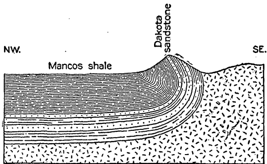
FIGURE 43.—Overturned eastern rim of the syncline at Crookton. Dakota sandstone dips steeply to the southeast.
