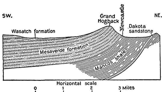
FIGURE 36.—Section through Grand Hogback at Newcastle.
