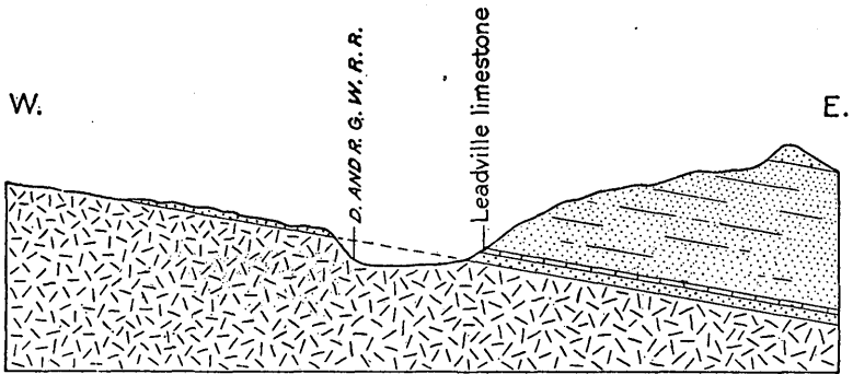
FIGURE 28.—Section across Eagle Park, showing the thin cap of quartzite on the west (left) and the same bed dipping into the base of the slope on the opposite side. The beds dip eastward, away from the Sawatch or Holy Cross anticline.
