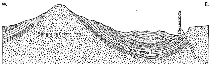
FIGURE 17.—Cross section of the Sangre de Cristo Range and the valley on its east side at Pleasanton, showing the anticline of the mountain and the syncline on the east.
