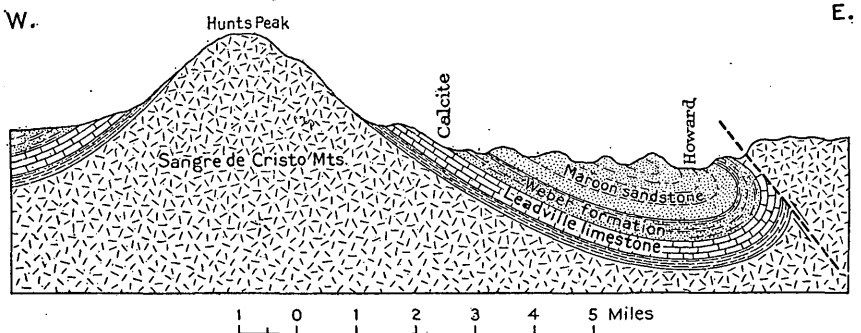
FIGURE 19.—Section of the Sangre de Cristo Range and the valley on its east side, through Hunts Peak and Howard.
